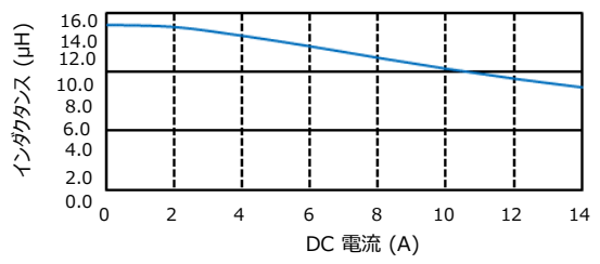
[ ETQP6M150KLC ]
