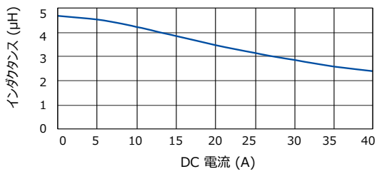
[ ETQP6M4R7YLC ]
