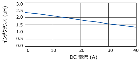
[ ETQP6M2R5YLC ]
