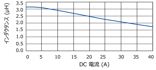
[ ETQP6M3R3YLC ]
