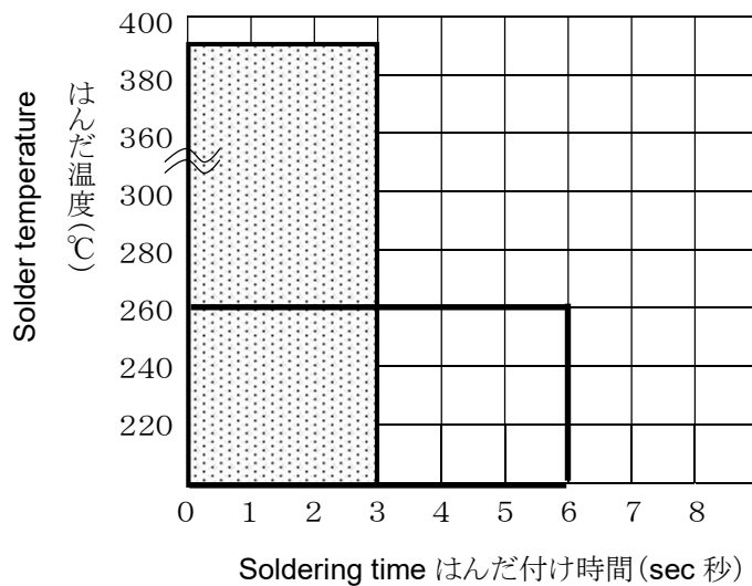
Fig. 5 Recommended soldering condition
