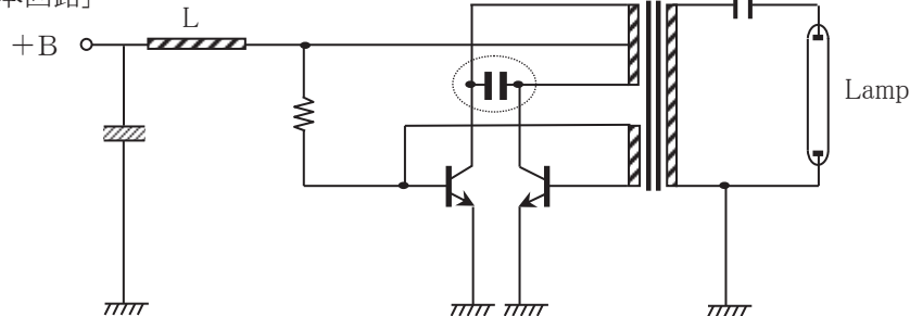
[基本回路]
