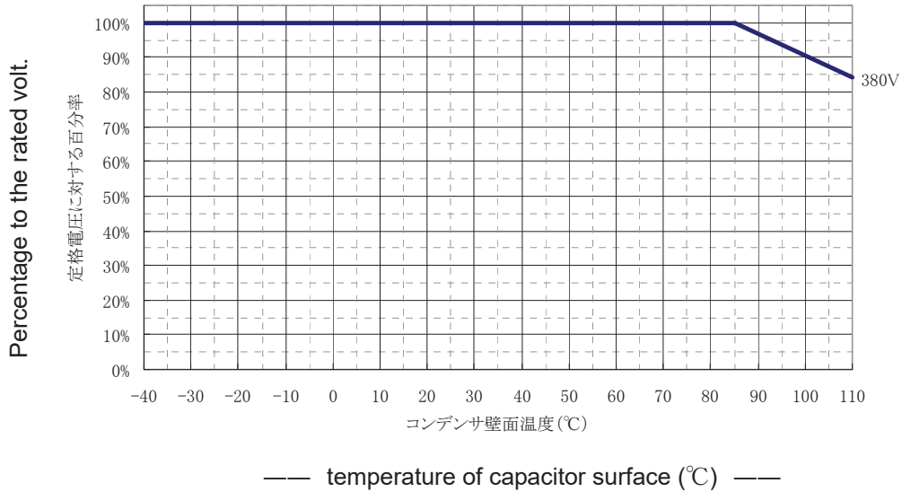
Fig.2 CURRENT DERATING VS. TEMPERATURE
