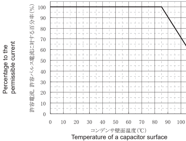
Fig.2 PERMISSIBLE TEMPERATURE RISE DERATING VS. SURFACE TEMPERATURE OF A CAPACITOR
