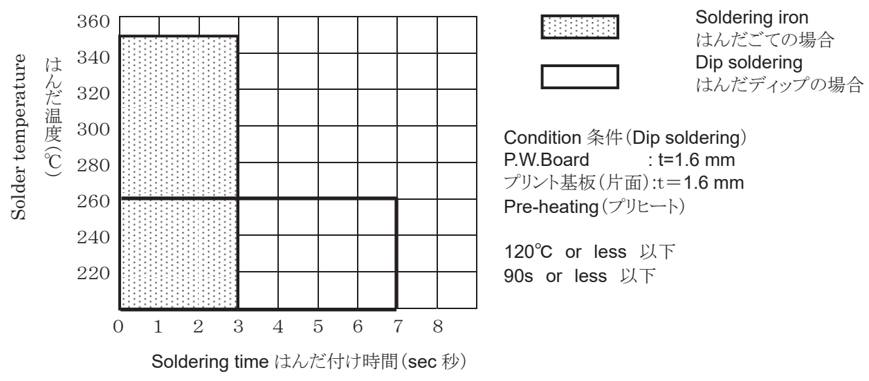
Fig. 4 Recommended soldering condition 図-4 推奨はんだ付け条件
